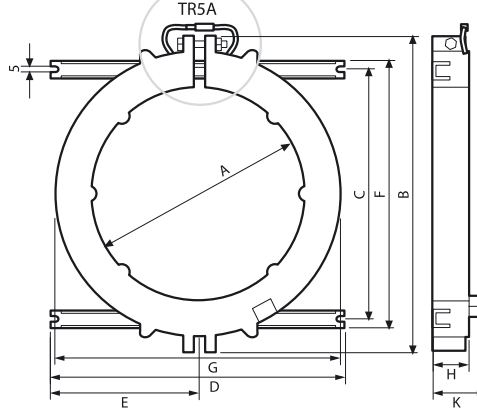
TR5, TR5A
