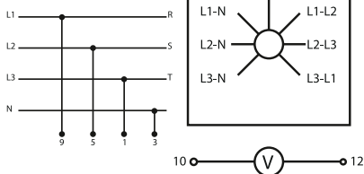
MCV7
