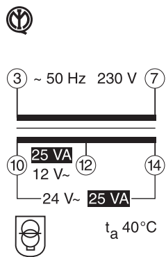
TS25/12-24 C
