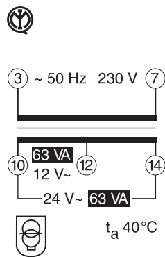
TS63/12-24 C
