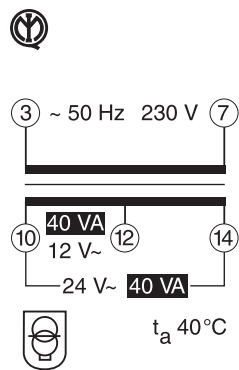
TS40/12-24 C
