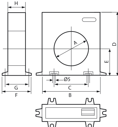
TR5, TR5A
