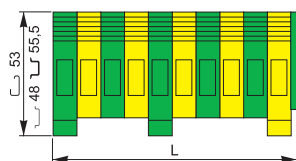
MB 10/10.P....
