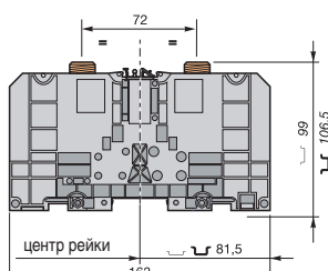
D 300/55.FF
