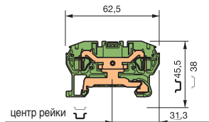
D 4/6.P.2L
