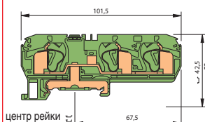
D 10/10.P...3L
