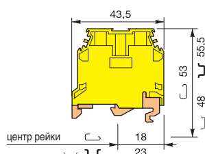
M 10/10.P
