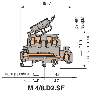
M 4/8.D2.SF
