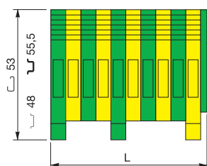
MB 4/6.P....
