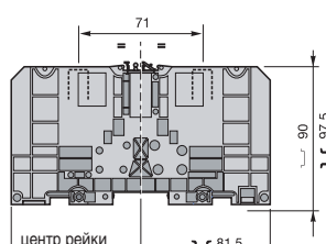
D 185/55.FF
