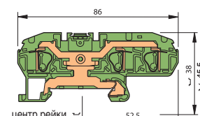
D 6/8.P...3L
