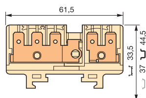
HD 6/9.3G.2G
