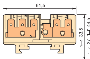
HD 6/9.2G.3G
