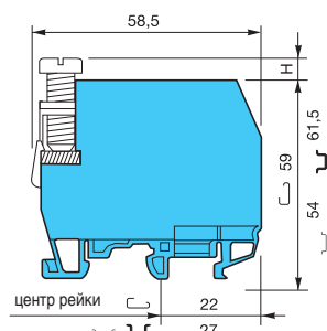
M 35/16.NT
