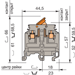
M 4/6.SNB
