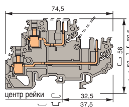
MA 2,5/5D2.2CPE
