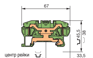
D 6/8.P...2L
