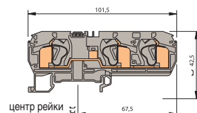
D 10/10...3L
