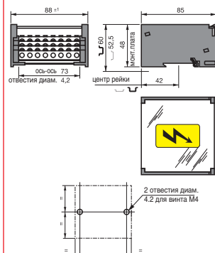
BRT 80 A
