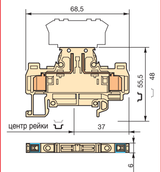
D 2,5/8.S.ADO.NF
