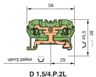
D 1,5/4.P.2L
