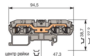
D 4/6.4L
