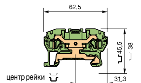
D 4/6.P.2L
