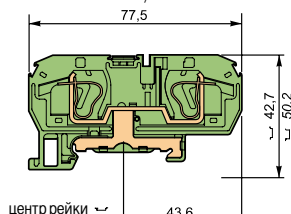
D 10/10.P.2L
