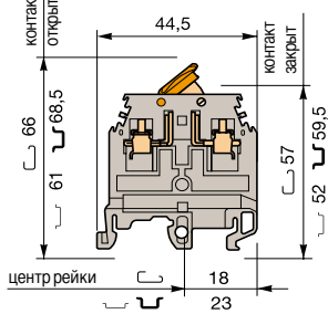
M 4/6.SNB
