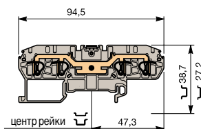
D 4/6.4L
