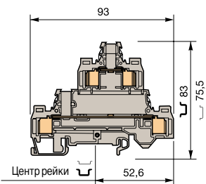
D 1,5/6.D2.ADO
