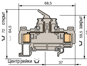
D 1/5.SNT2.ADO
