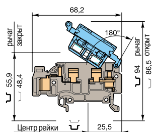
D 4/8.SNN.I.ADO
