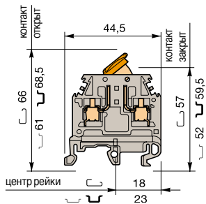
MA 2,5/5.SNB
