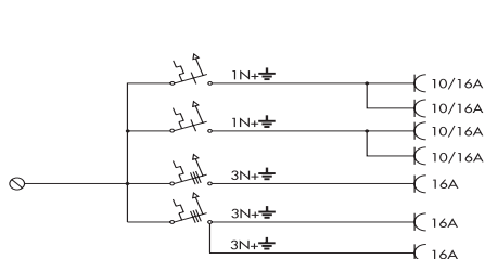
MPR16/3
