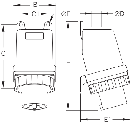
263-463BS...W
