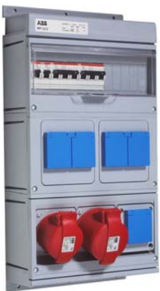
MP 32/2
