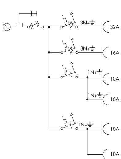
M 32/2 JFB
