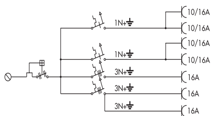
MP16/3
