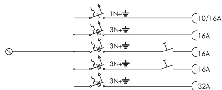
MP 32/SW2
