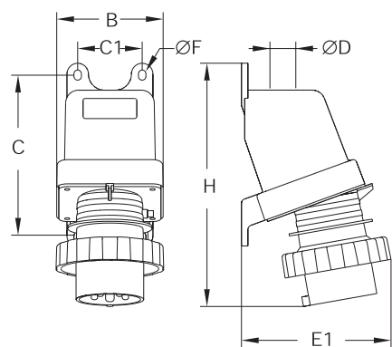
216-432BS...W
