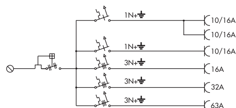
MPR 63/1
