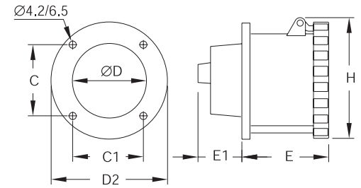
263-4125RU...W
